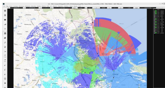
Best server coverage
